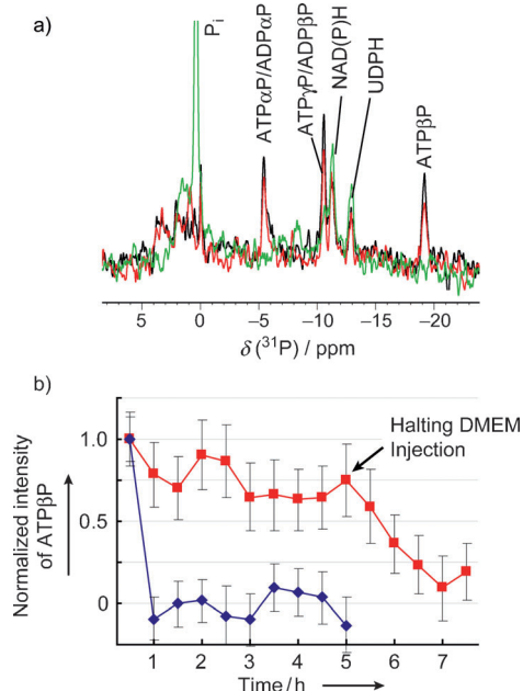
Figure 2. a) ^{31}\text{P} NMR spectra of freshly harvested HeLa cells were acquired immediately (black), after 30 min incubation in DMEM (green), and after 5 h incubation in the bioreactor (red). b) Time course of the signal intensity originating from the \beta P atom of intracellular ATP, with (red) and without (blue) the bioreactor. The injection was stopped at the time point indicated by the arrow. The error bar is the signal-to-noise ratio for each spectrum.
