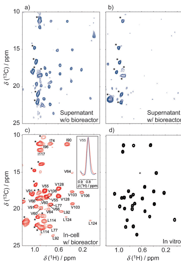
Figure 3. ^1\text{H} - ^{13}\text{C} methyl-TROSY spectra of supernatant collected after in-cell NMR experiments after 1 h incubation in the absence of the bioreactor (a) and after 4.5 h incubation in the bioreactor (b). c) ^1\text{H} - ^{13}\text{C} methyl-TROSY spectrum of the CG1-treated cells acquired after 5 h incubation in the bioreactor. The in-cell NMR spectrum in the absence of the bioreactor was measured 15 min before signals of the leaked protein were detected in the supernatant. Asterisks indicate signals from the components of the cell and the medium (Figure S10 in Supporting Information). For comparison of the linewidths, the inset shows the signal corresponding to V55 in the in-cell 1D NMR spectra, with (red) and without the bioreactor (blue). d) ^1\text{H} - ^{13}\text{C} methyl-TROSY spectrum of purified CG1.
